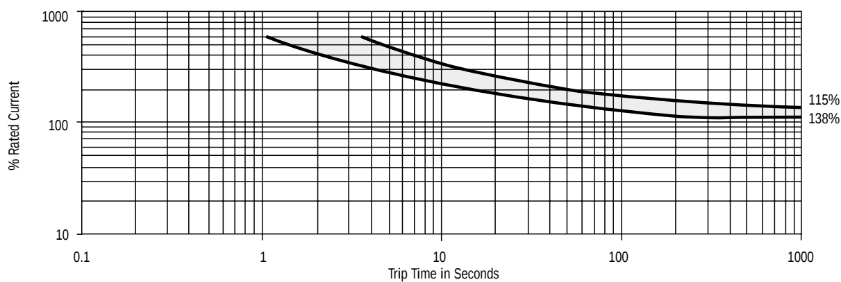
Approximate Time-Current Curve 3TC7 Circuit Breakers
